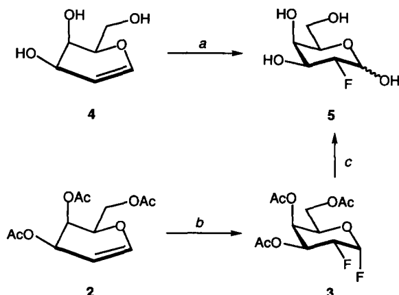
Scheme 1. (a) XeF_2 (1.8 equivalents), H_2O , rt, 1.5 h, 30%, \alpha:\beta=1:1.5 . (b) XeF_2 , BF_3 \cdot Et_2O , Et_2O -benzene, rt, 2.5 h, 78%. (c) 2 N HCl, 90 °C, 2 h, 83%, \alpha:\beta=1:1.6 .
