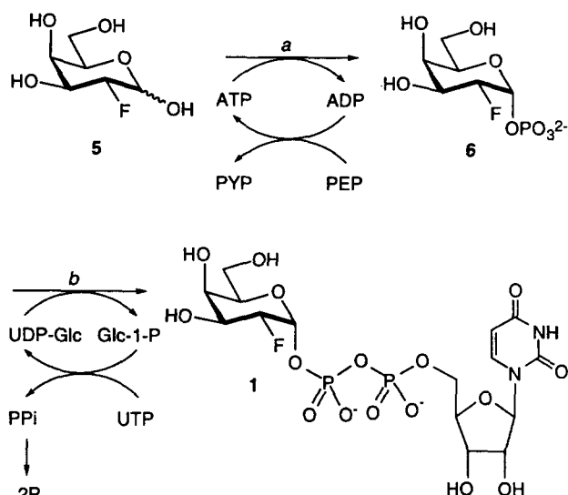
Scheme 2. (a) Galactokinase, pyruvate kinase, ATP:Na 3 , phosphoenolpyruvate:Na 3 (PEP:Na 3 ), dithiothreitol, cysteine, Mg 2+ , Mn 2+ , K + , HEPES 100 mM, pH 7.4, four days under Ar, rt, 58%. (b) Galactose-1-phosphate uridylyltransferase, UDP-glucose (UDP-Glc), pyrophosphorylase, pyrophosphatase, UTP:Na 3 , UDP-Glc:Na 2 , dithiothreitol, pH 8.4, two days under Ar, rt, 67%.
