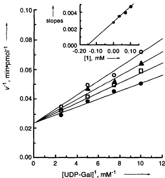
Figure 1. Inhibition kinetics of \beta -1,4-galactosyltransferase with UDP-2FGal 1 with respect to UDP-Gal in the presence of N -acetyl-D-glucosamine (GlcNAc) (1.0 mM) and Mn 2+ (1.0 mM) in HEPES (100 mM, pH 7.4). The concentrations of inhibitor 1 were 0 mM (●), 0.035 mM (□), 0.070 mM (▲), and 0.105 mM (○). Inset: secondary plot of slopes obtained from the double reciprocal plots versus [1].
